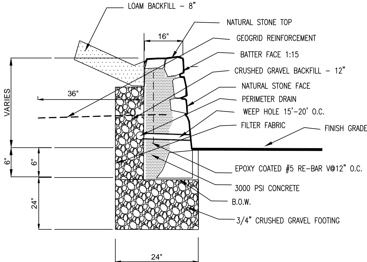
R-1 TYPICAL RETAINING WALL 2-4 FEET NOT TO SCALE
