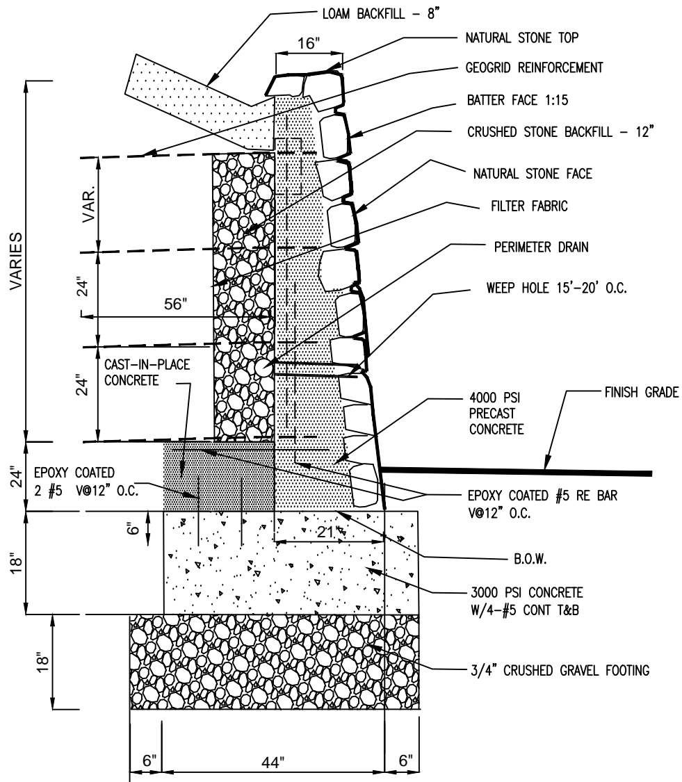
R-1 TYPICAL RETAINING WALL 6-8 FEET NOT TO SCALE
